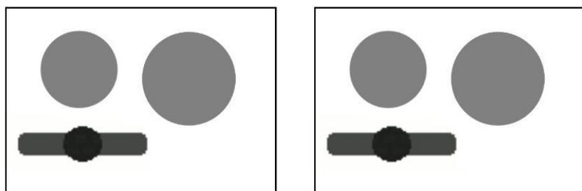
Arm joints
